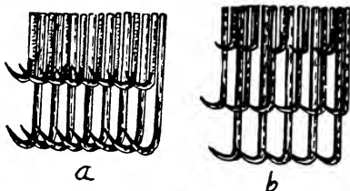
Fig. 473. a, Biordinal crochets; b, triordinal crochets.
